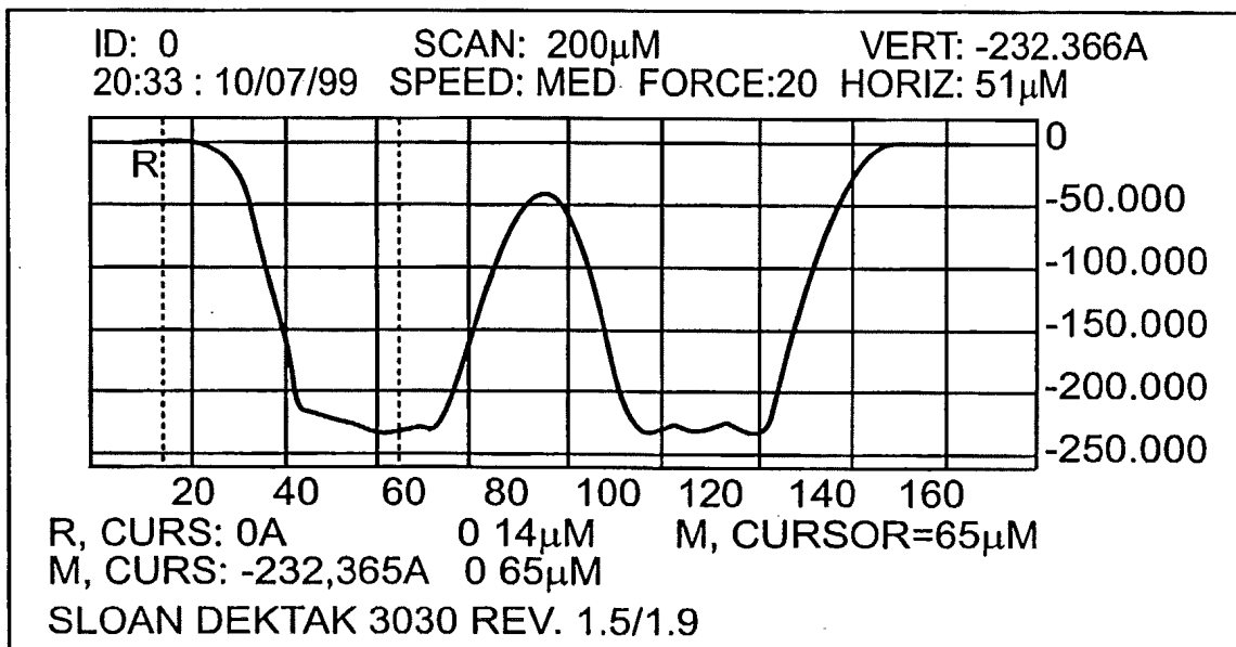
SURFACE TOPOGRAPHY SCANS FOR THE ANNULI OF FIG. 11
